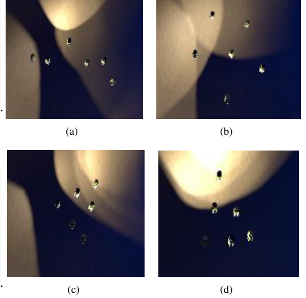
Fig. 12. Simulation of building pyramid pattern. (a) starting state of six vehicles, (b) intermediate CP from (a), and (c),(d) two pyramid patterns built, (c) based on the intermediate CP (b), and (d) according to the PCA from (a).
