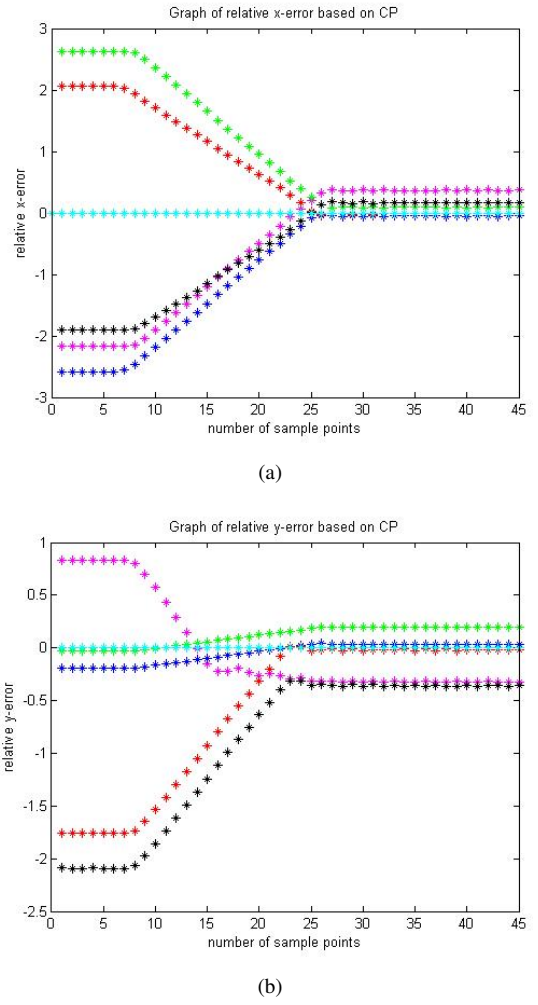
Fig. 14. Relative errors between (x_a, y_a) and (x_d, y_d) based on CP: (a) relative x-errors; (b) relative y-errors. The points are sampled by taking one point every 100 points from original data.
