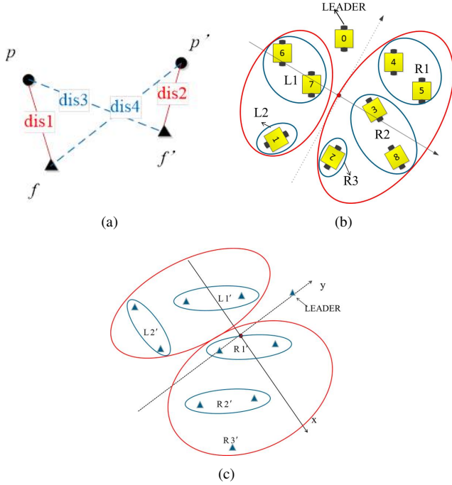
Fig. 5. Illustration of control algorithm for CA. (a) Matching up with shorter distance for CA. (b), (c) an example sketch of strategy based on PCA: (b) division of initial group and (c) division of final group in pyramid.
