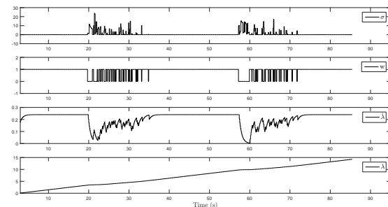
Fig. 9. SMRC signals
