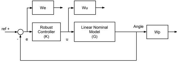
Fig. 4. H_\infty synthesis structure: weighting functions, nominal model, controller.
