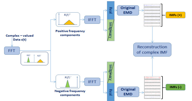
Fig. 1. Block diagram of CEMD algorithm.
