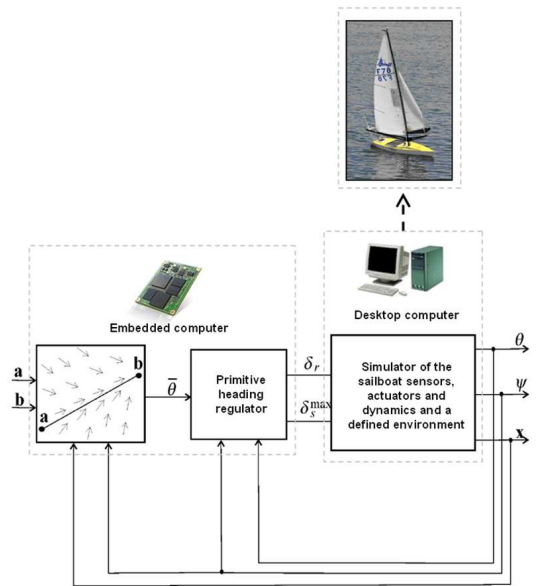
Fig. 9. HWIL architecture
