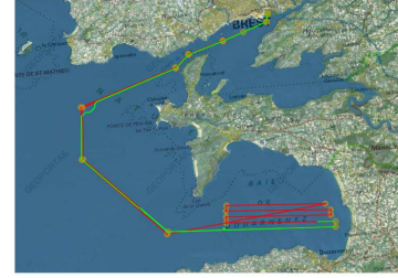
Fig. 8. Trajectories: objective in red and realized in green
