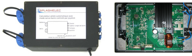
Fig. 2 PSC of the Splashelec system in a waterproof case. It contains several inputs for the keyboard, the compass, the rudder angle sensor, the battery...
