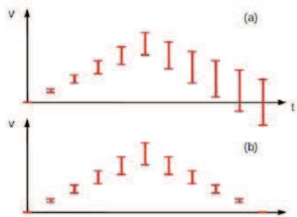
Figure 10. Representation of the speed intervals (a) with a forward-only algorithm (b) with a forward-backward algorithm.
