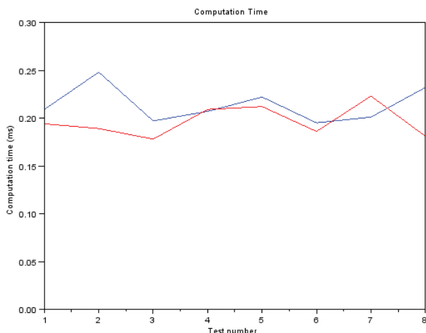
Figure 11. Performance tests. RANSAC in red. Forward-Backward in blue.
