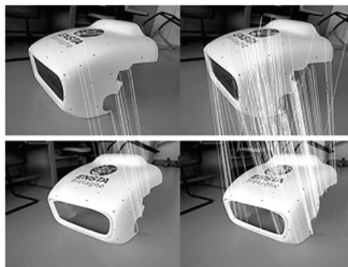
Figure 3. Comparison of the number of correspondences found on a mechanical prototype. SIFT is on the left and A-SIFT is on the right.
