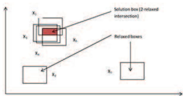
Figure 8. Set inversion on outliers generates empty intersections. We have to relax them to obtain the solution.
