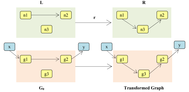
Figure 2. Preservation of the property GraphPath ( x,y ) after the application of the rule r on the graph G_0 . The r 's right graph R satisfies GraphPath ( n1,n2 ).
