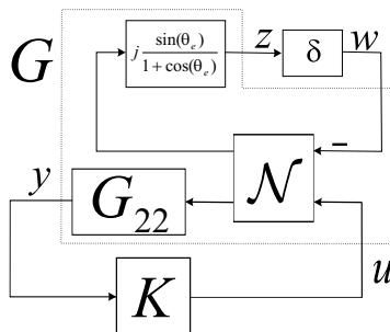
Figure 9: Closed-loop structure for phase margin specification.
