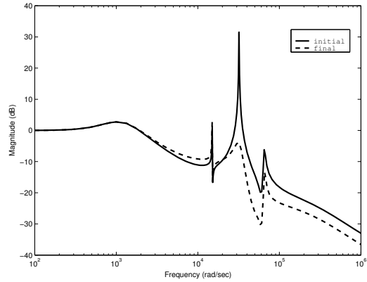
Figure 11: Reduction of the resonance peak (flexible model)
