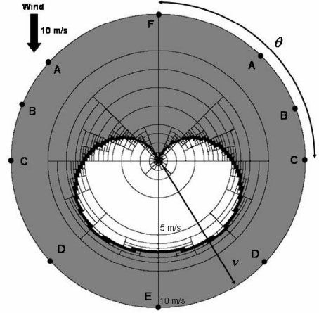
Fig. 4. Polar diagram obtained with QSI solver.
