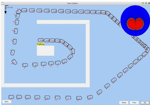
Fig. 5. Required manoeuver to moor the sailboat inside a harbor.
